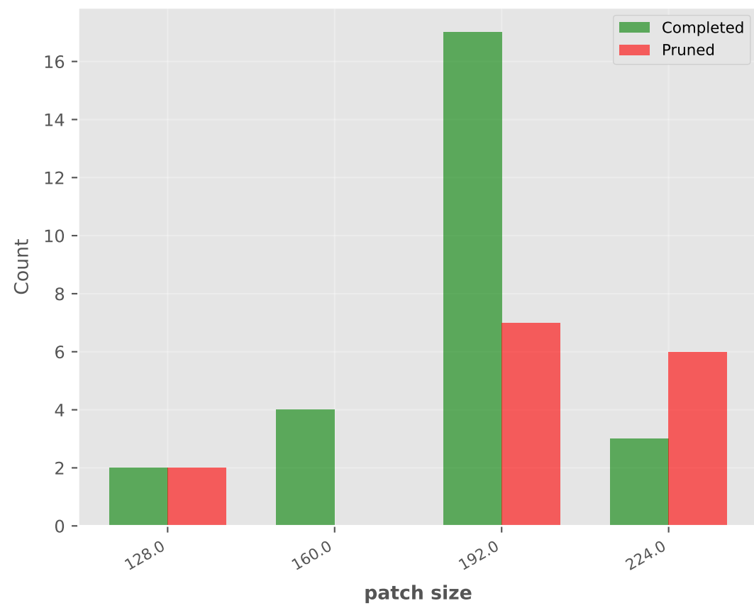
patch size: Completed vs Pruned
