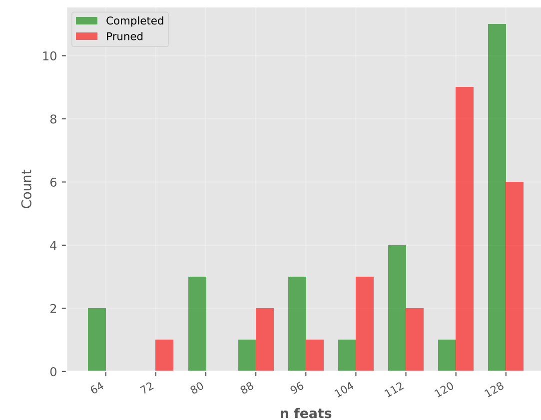
n feats: Completed vs Pruned
