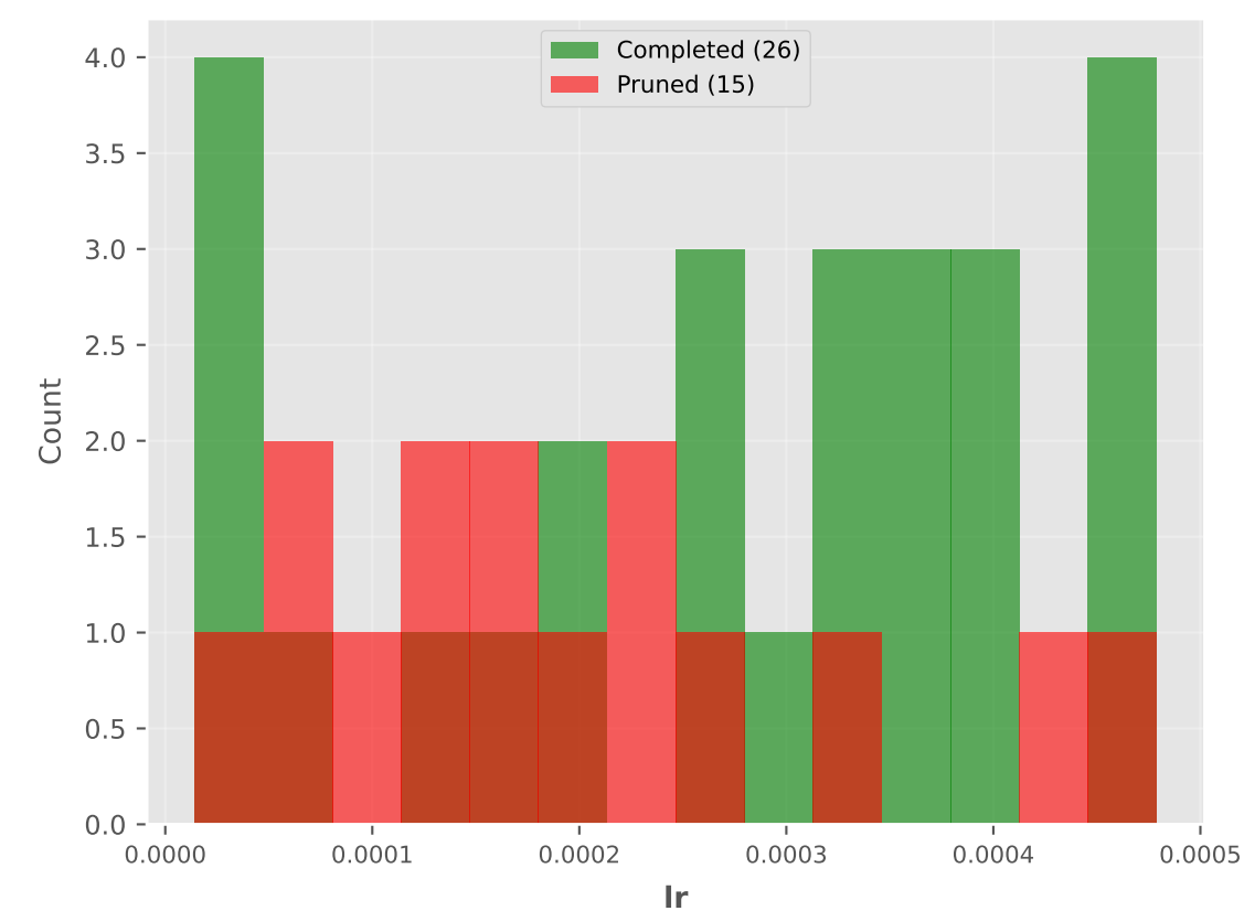
lr: Completed vs Pruned
