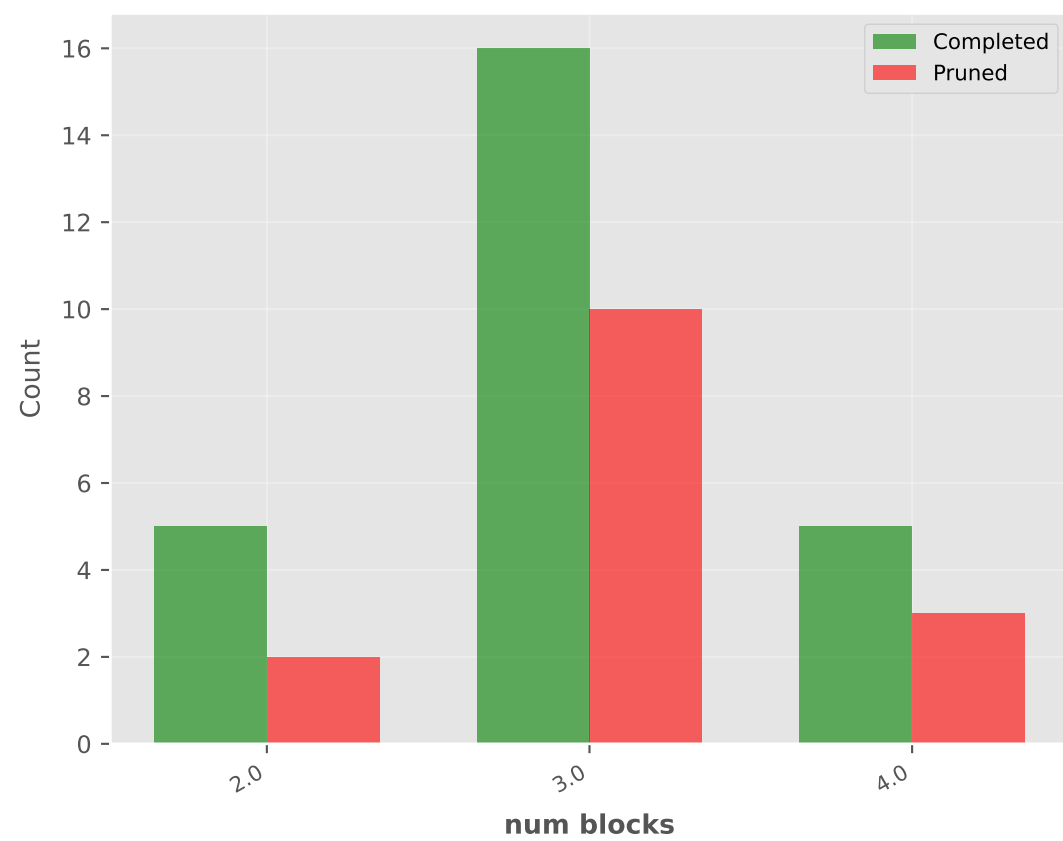
num blocks: Completed vs Pruned
