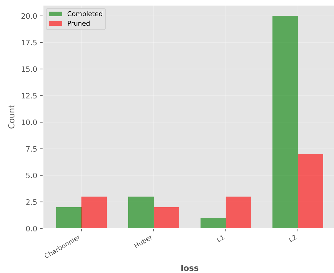
loss: Completed vs Pruned
