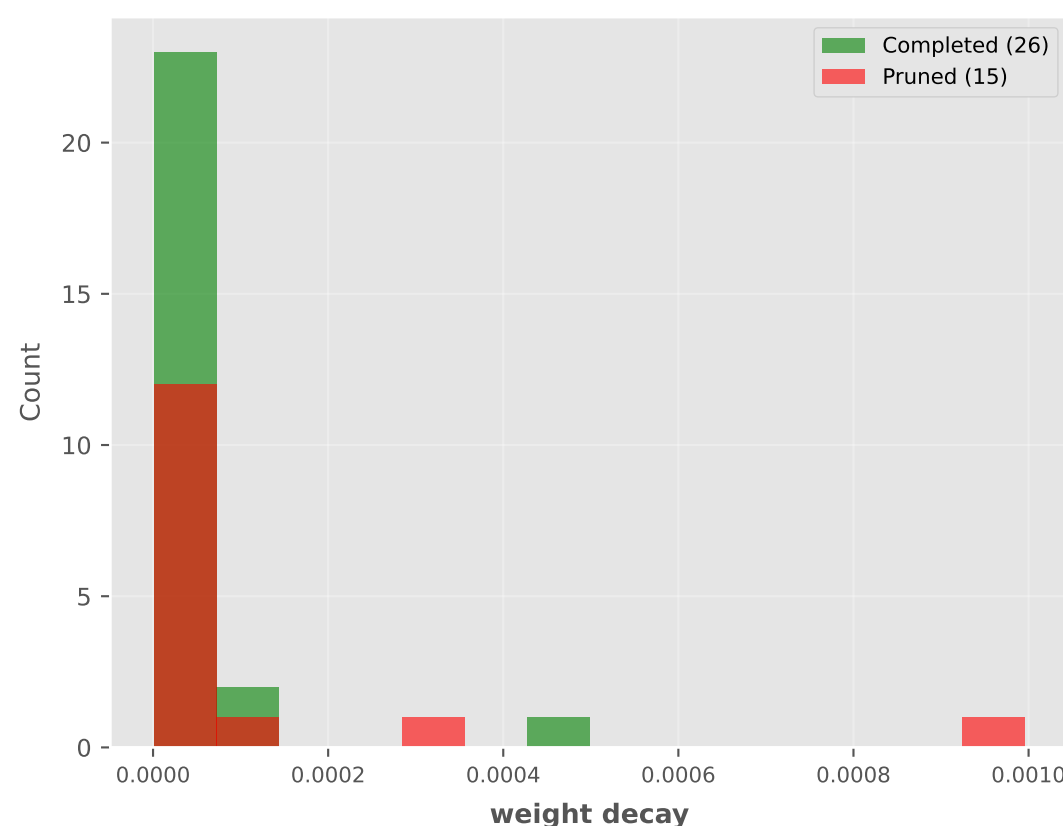
weight decay: Completed vs Pruned
